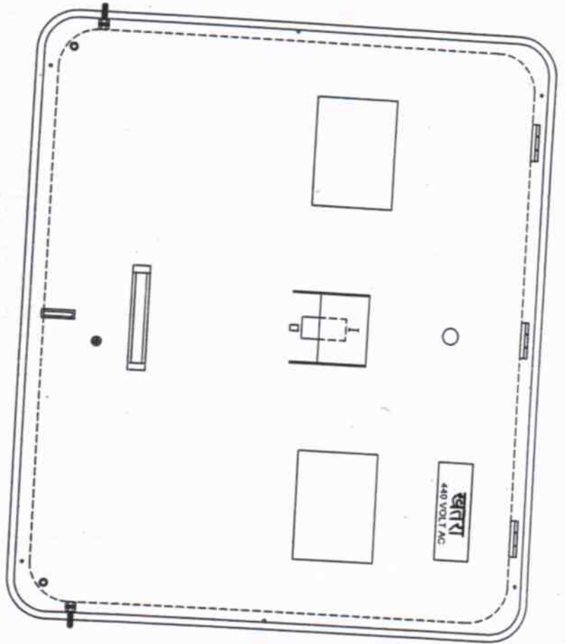
ELEVATION WHEN DOOR CLOSED
