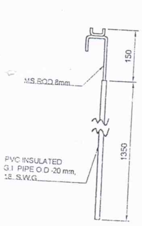
OPERATING ROD
